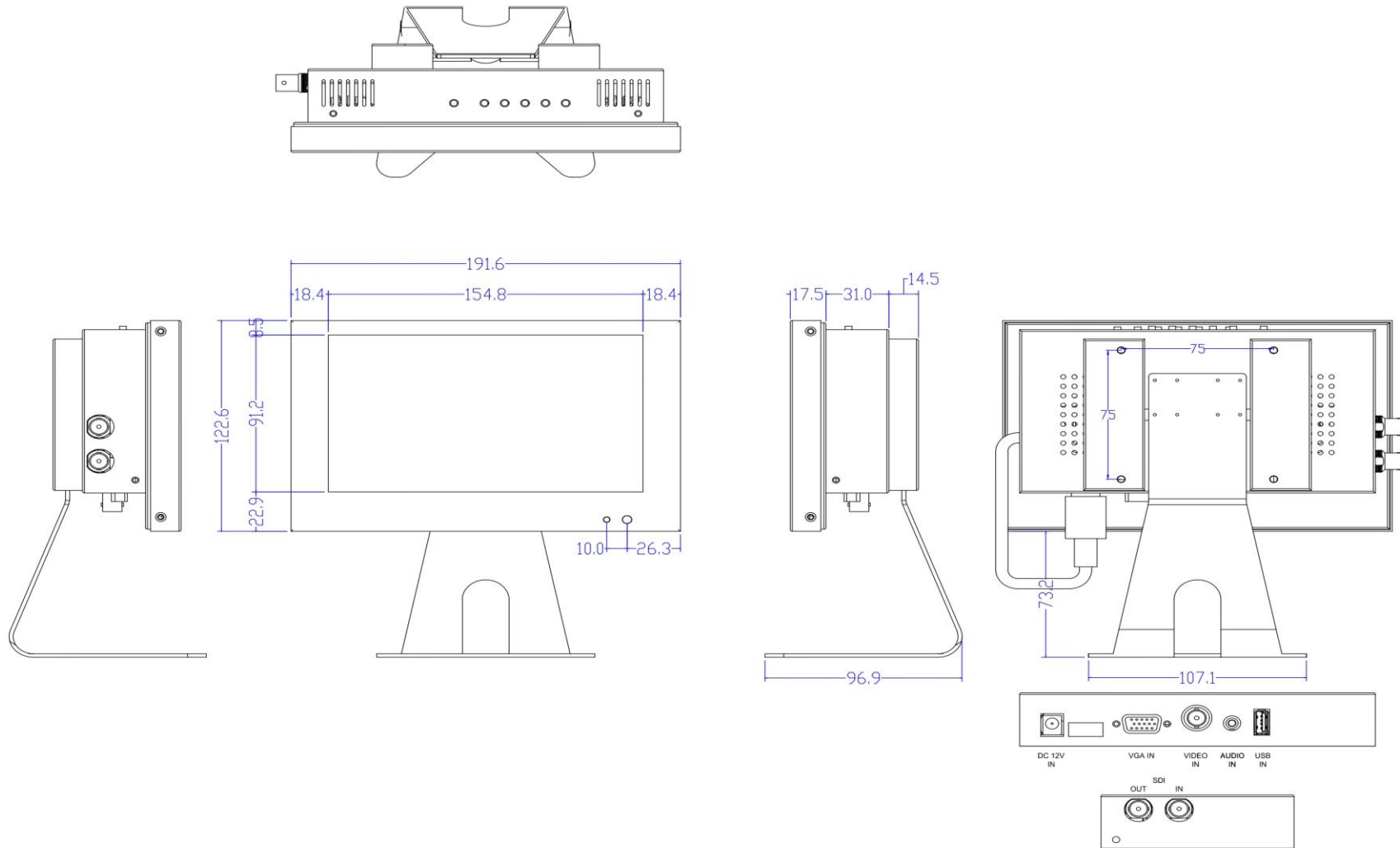
Line Drawing for: Model No. L70HSDI All sizes are in mm Drawing not to scale.
