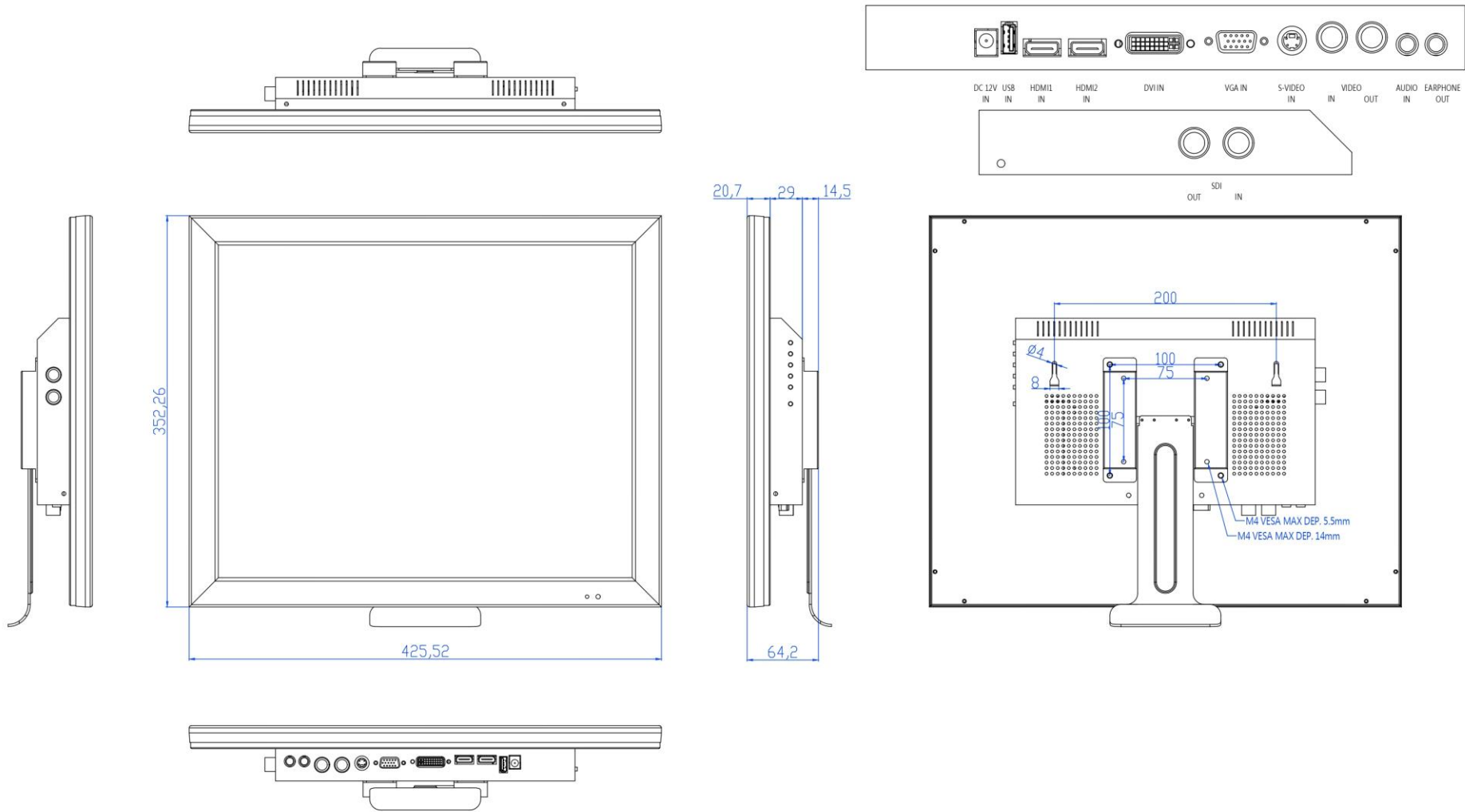
Line Drawing for: Model No. L192HMSDI All sizes are in mm Drawing not to scale.
