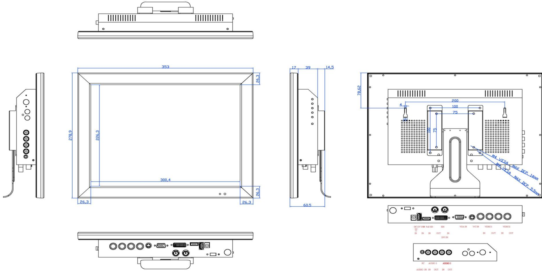
Line Drawing for: Model No. L152SDI All sizes are in mm Drawing not to scale.
