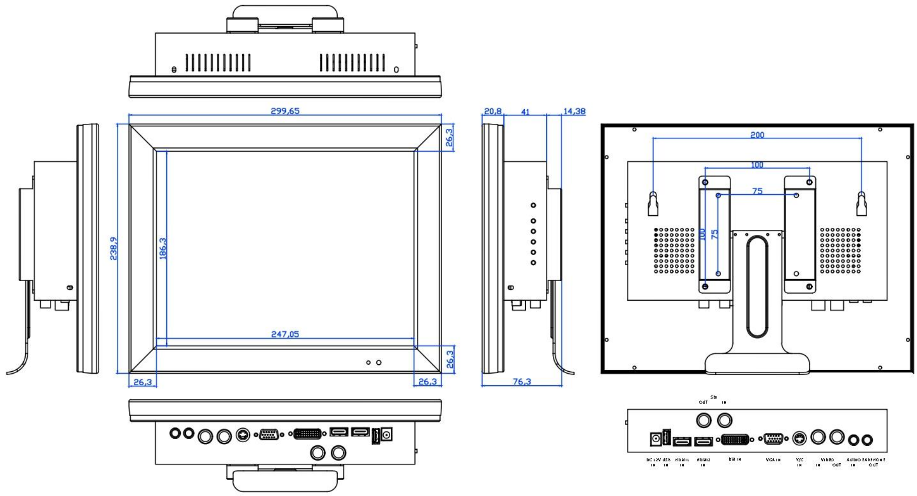
Line Drawing for: Model No. L121HMSDI All sizes are in mm Drawing not to scale.
