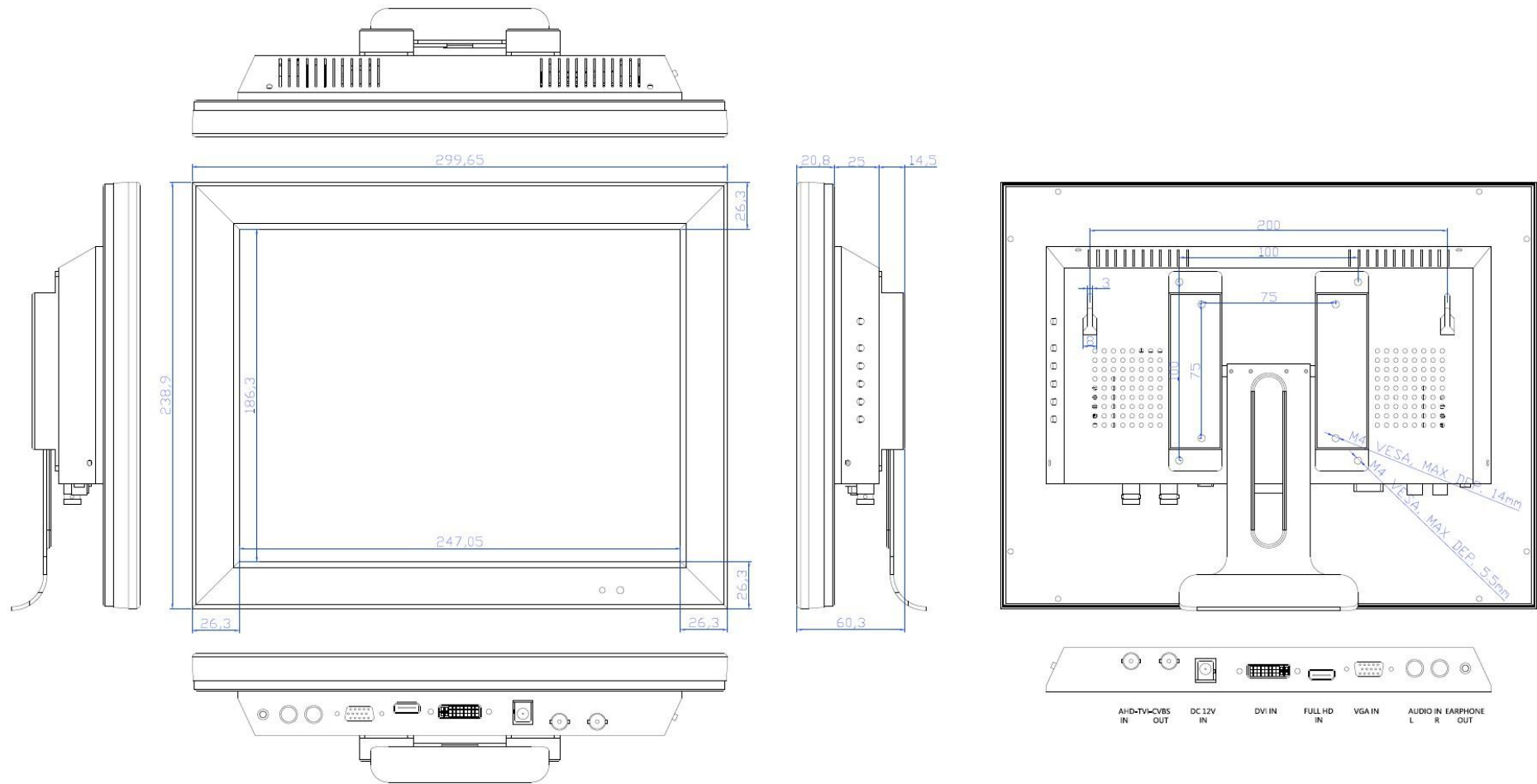
Line Drawing for: Model No. L121ATC All sizes are in mm Drawing not to scale.
